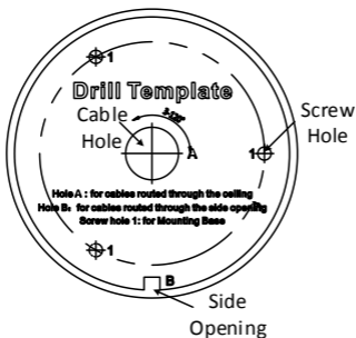
Figure 2-1 Drill Template
