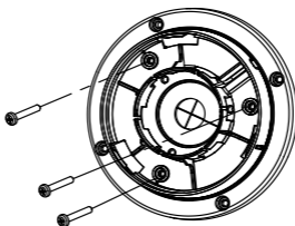
Figure 2-6 Install Turret Camera's Mounting Base
